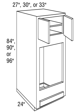
Double Oven Cabinets, 24" Deep
